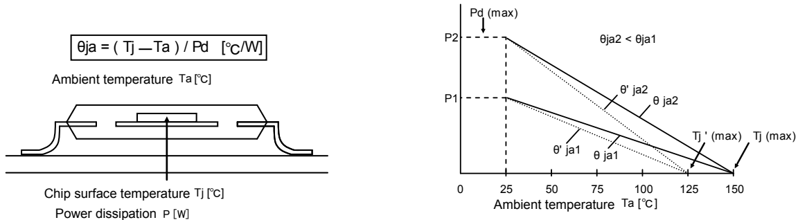
(a) Thermal resistance (b) Derating curve Fig.91 Thermal resistance and derating curve
