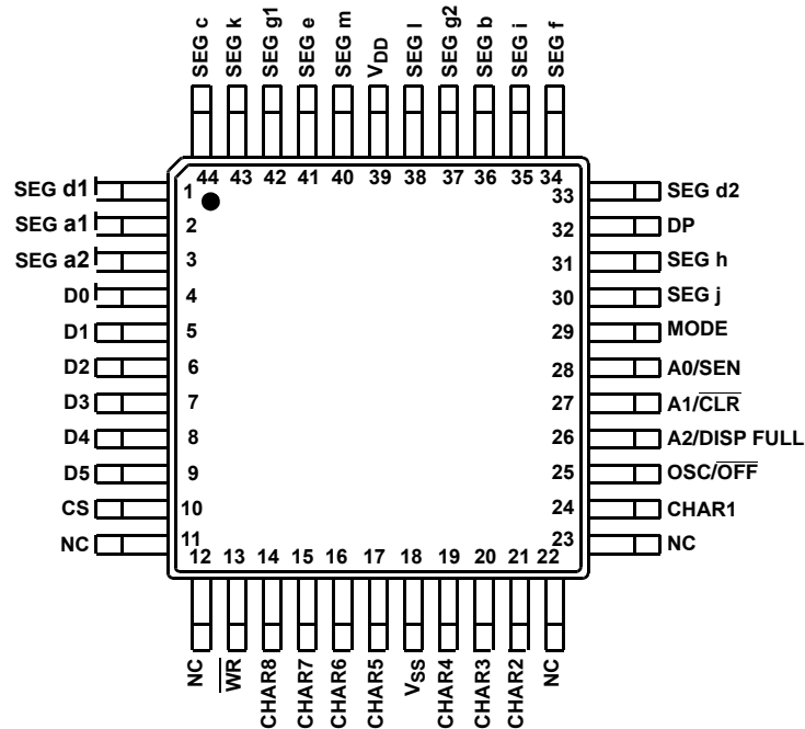
ICM7243A (16-SEGMENT CHARACTER) (MQFP) TOP VIEW
