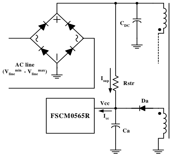
Figure 4. Startup circuit
