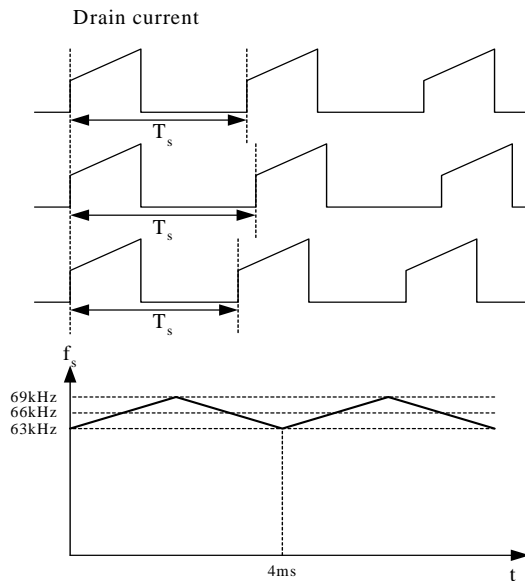
Figure 9. Frequency Modulation
