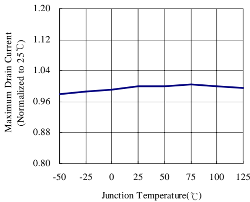
Maximum Drain Current vs. Temp
