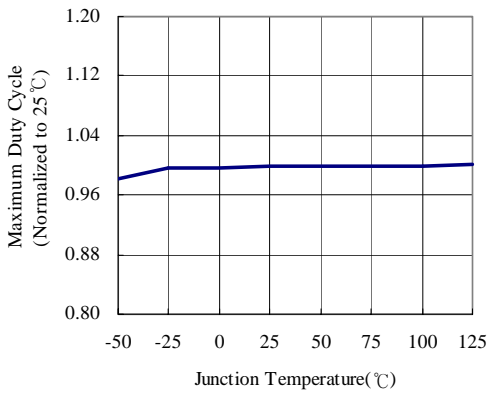
Maximum Duty Cycle vs. Temp
