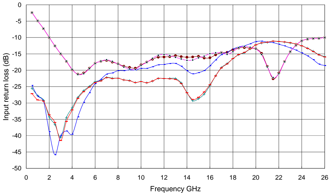
Input Return Loss versus attenuation states
