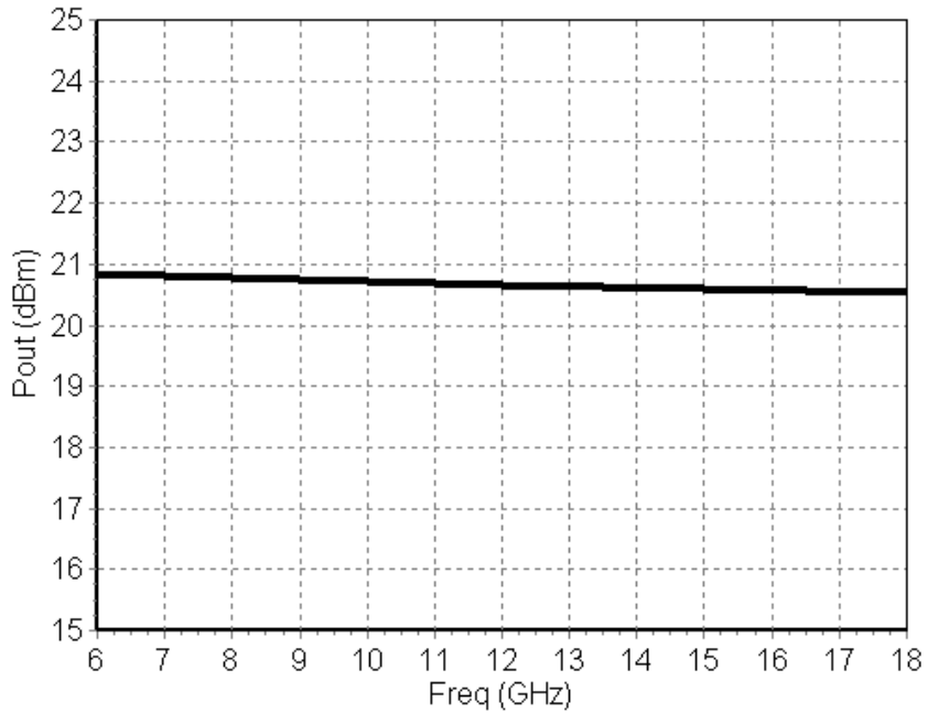
Saturated output power @ nominal state
