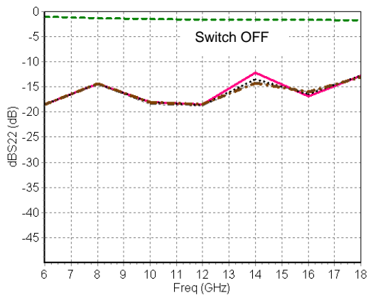
dB(S22) versus frequency for all states
