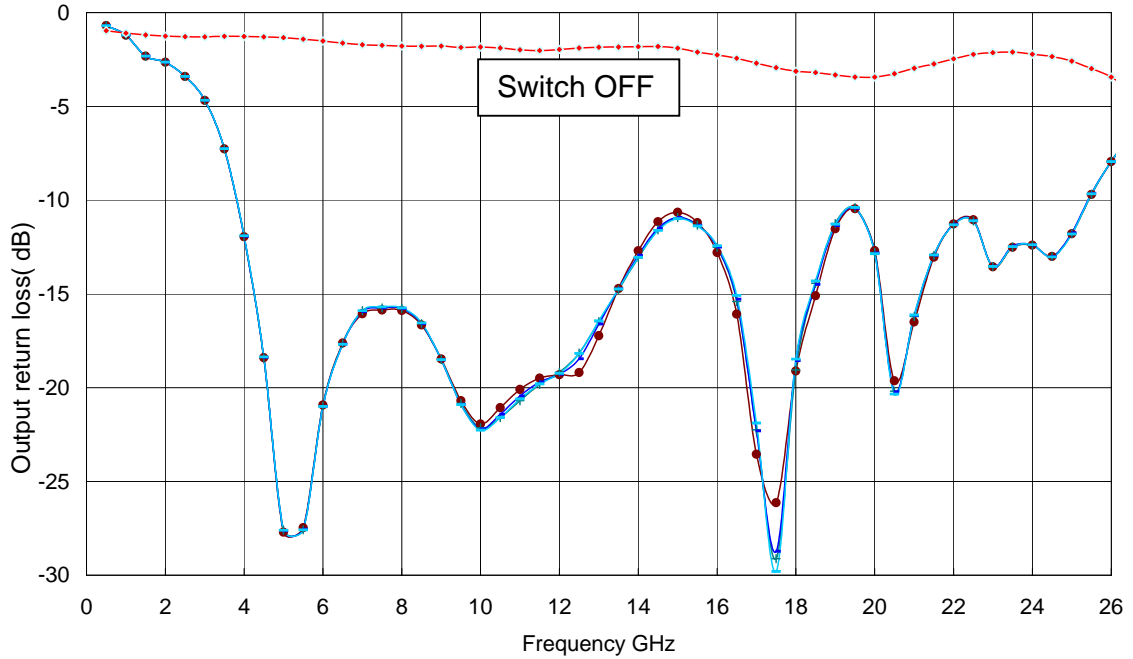
Output Return Loss versus attenuation states
