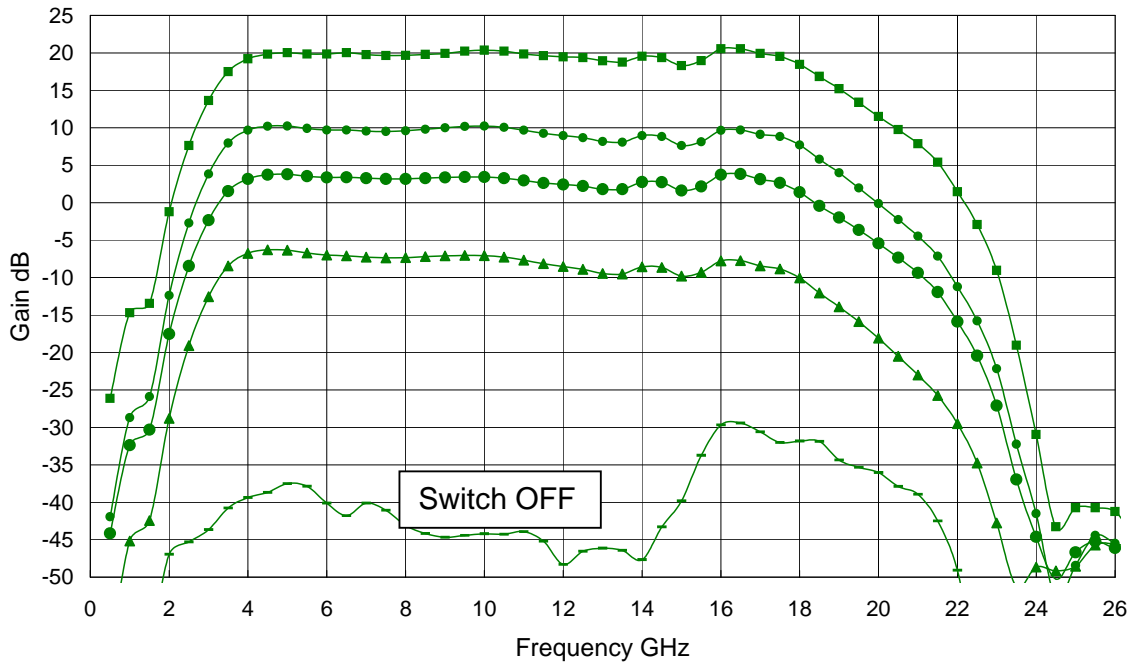
Linear Gain versus attenuation states
