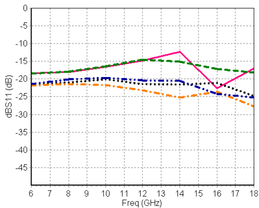
dB(S11) versus frequency for all state
