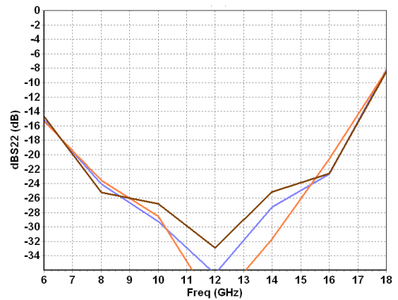
dB(S22) versus frequency for all states
