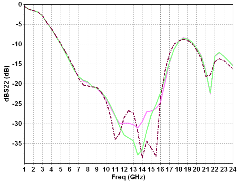
Output Return Loss versus attenuation states
