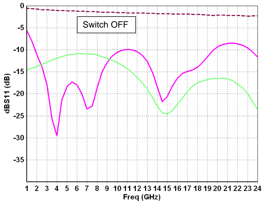
Input Return Loss versus attenuation states
