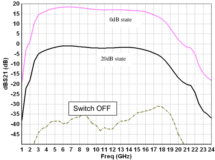
Linear Gain versus attenuation states
