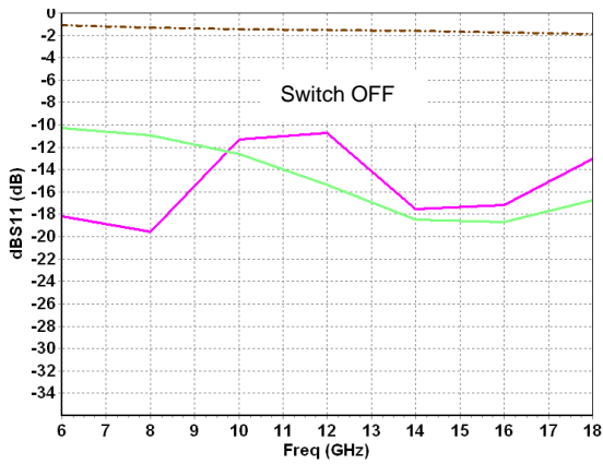
dB(S11) versus frequency for all states
