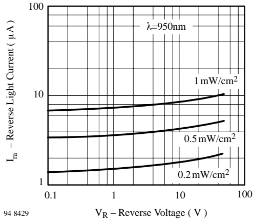
94 8429 Figure 4. Reverse Light Current vs. Reverse Voltage
