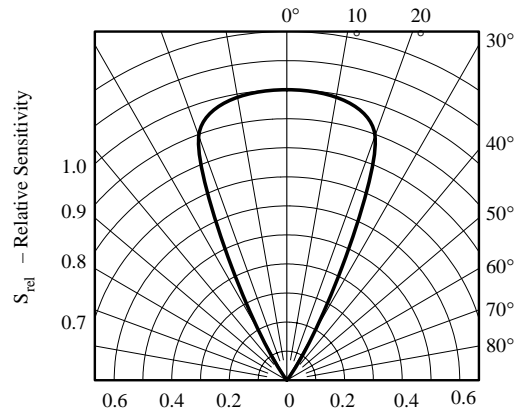
94 8431 Figure 7. Relative Radiant Sensitivity vs. Angular Displacement
