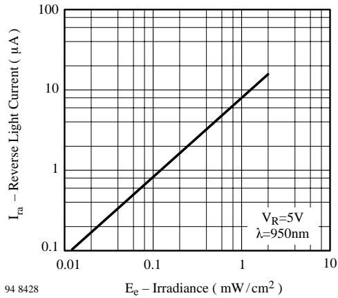
94 8428 Figure 3. Reverse Light Current vs. Irradiance
