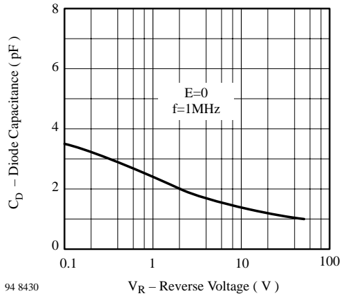
94 8430 Figure 5. Diode Capacitance vs. Reverse Voltage
