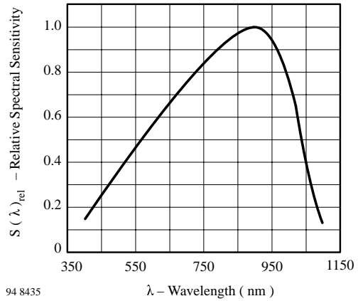
94 8435 Figure 6. Relative Spectral Sensitivity vs. Wavelength
