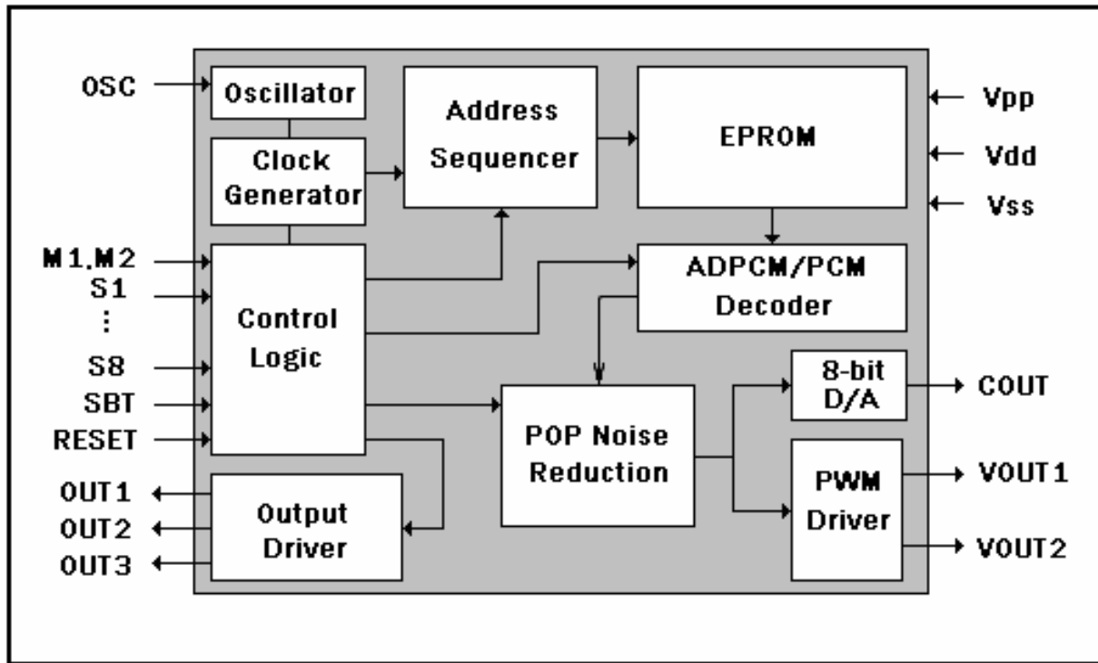
Fig. 17 Block Diagram
