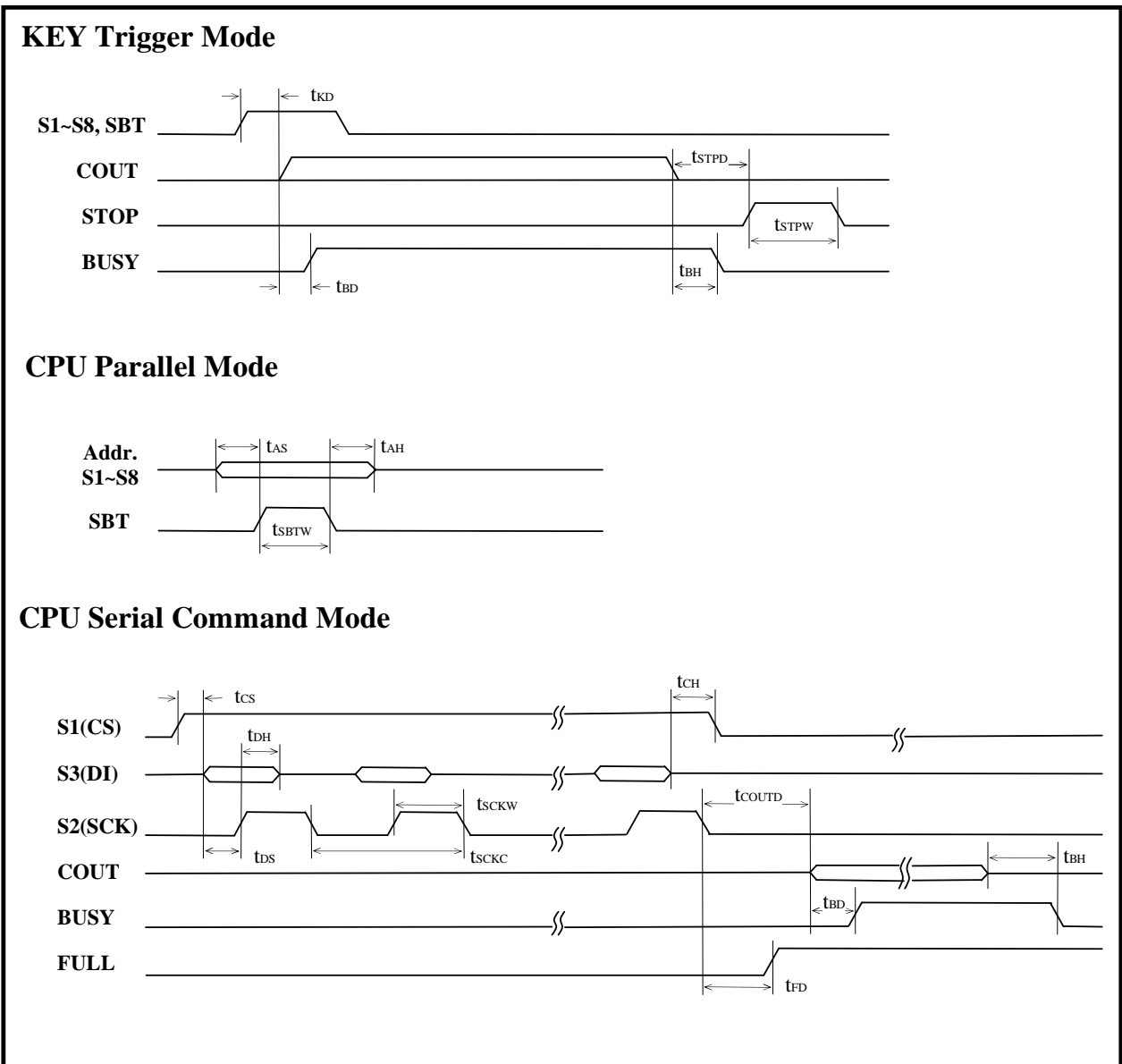
Fig. 18 Timing Waveform
