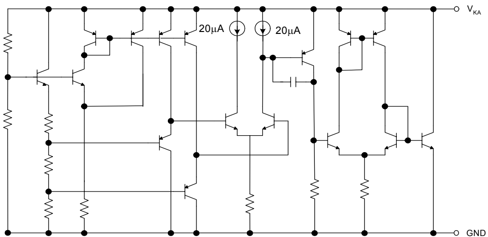
Figure 5. Voltage Reference Functional Block Diagram
