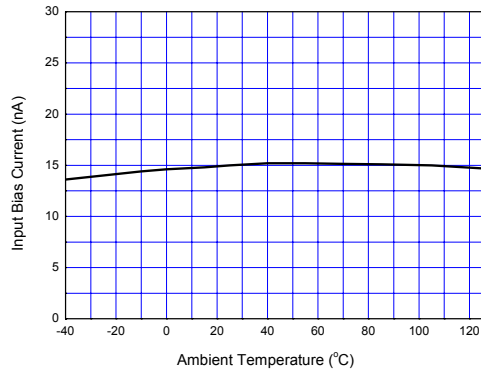
Figure 10. Input Bias Current vs. Ambient Temperature
