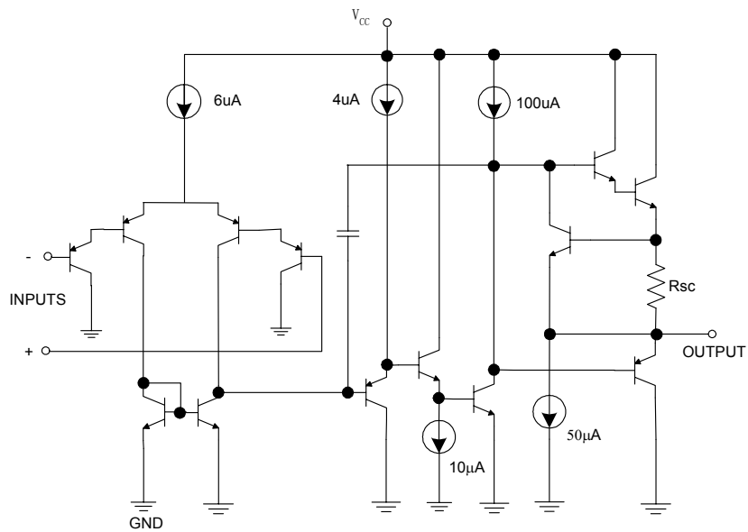
Figure 4. OPAMP Functional Block Diagram (Each Amplifier)
