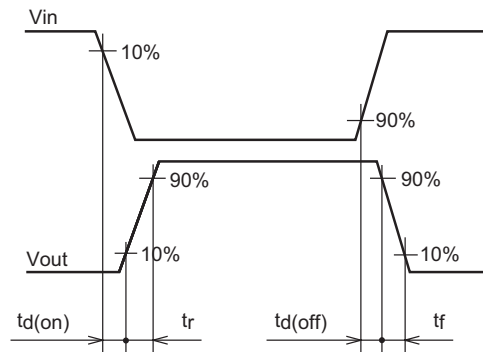
Switching Waveform
