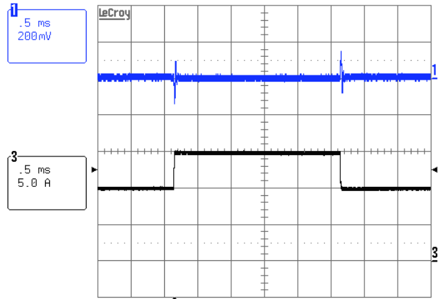
Figure 11. Vin=12V, Vout=2.5V
