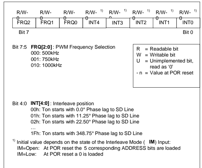
Figure 38. Interleave Configuration Register INT
