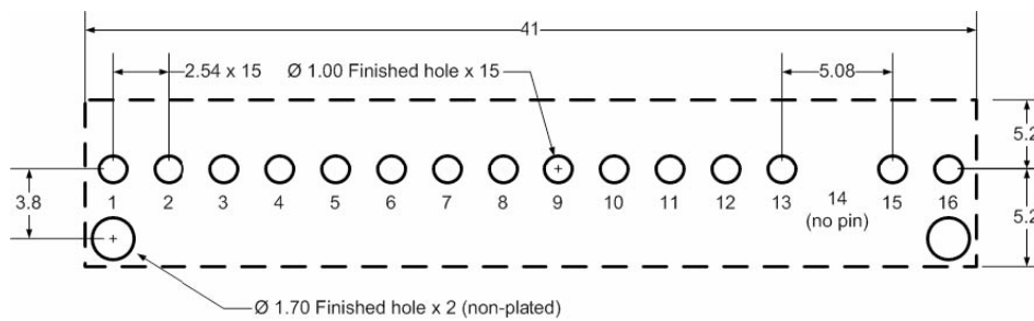
Figure 49. Recommended Footprint – Top View (all dimensions in mm)
