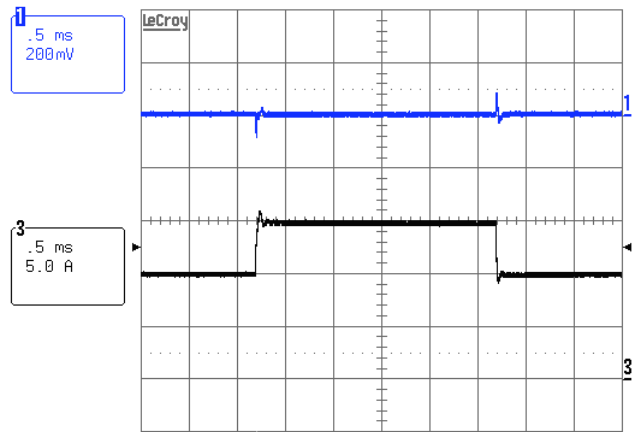
Figure 12. Vin=12V, Vout=0.5V
