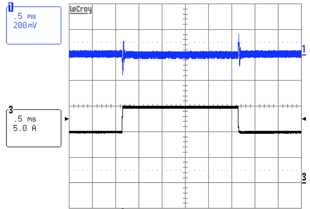
Figure 10. Vin=12V, Vout=5.0V
