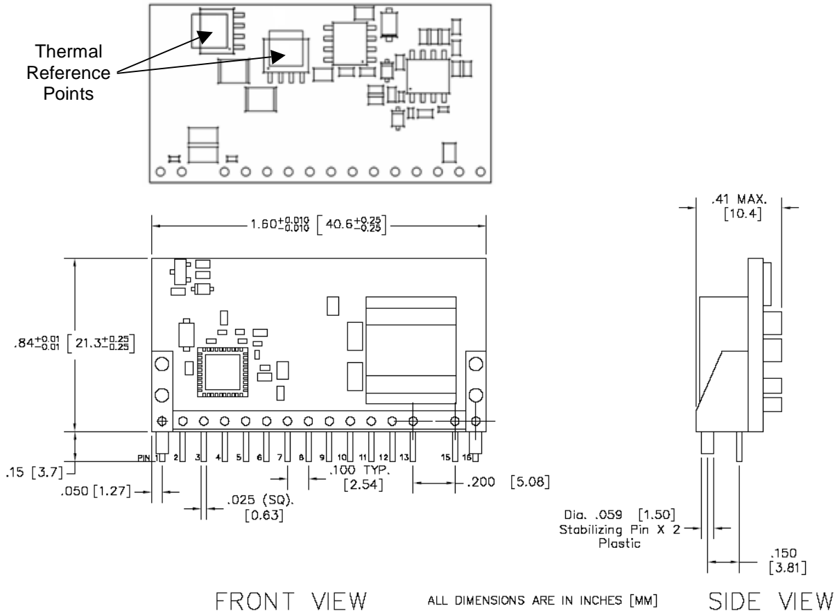
Figure 48. Mechanical Drawing
