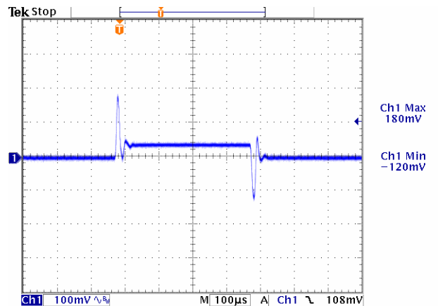
Figure 14. Vin=12V, Vout=1.0V
