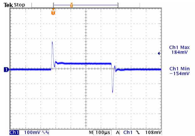
Figure 13. Vin=12V, Vout=2.5V
