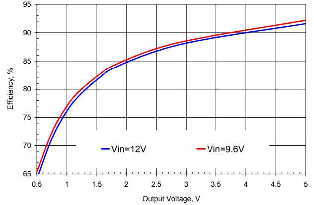
Figure 3. Efficiency vs. Output Voltage, Iout=10A, Fsw=500kHz
