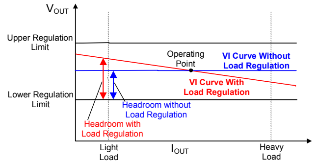
Figure 20. Concept of Optimal Voltage Positioning
