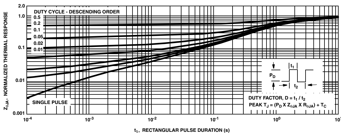
Figure 17. Normalized Transient Thermal Impedance, Junction to Case
