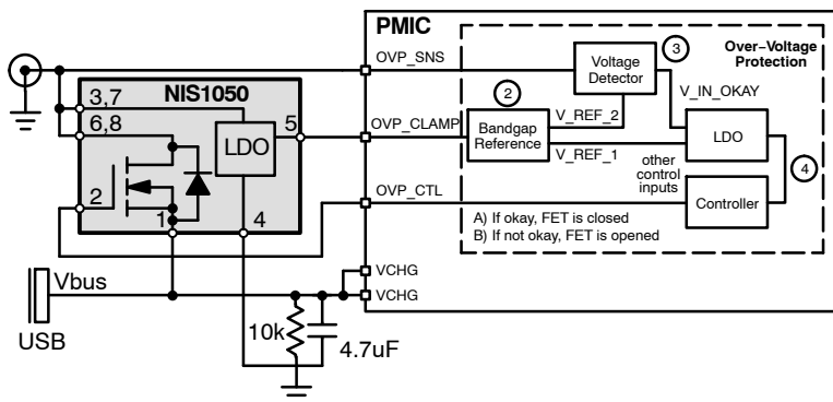
Figure 1. Typical Application
