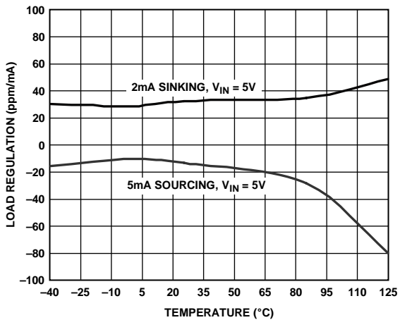
Figure 21. ADR121 Load Regulation vs. Temperature
