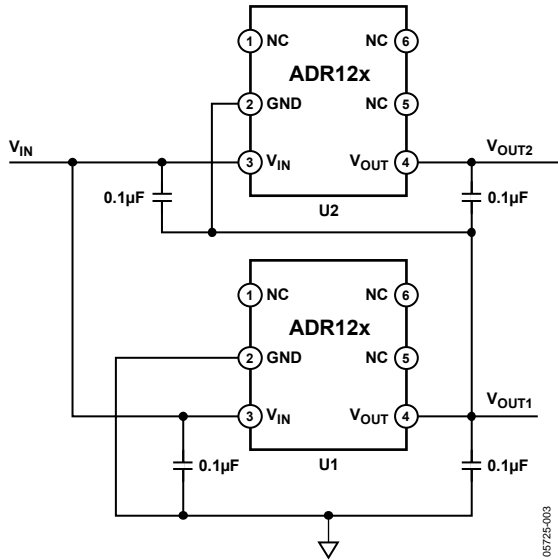
Figure 50. Stacking References with ADR12x
