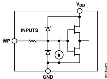
Figure 27. Equivalent \overline{\text{WP}} ESD Protection
