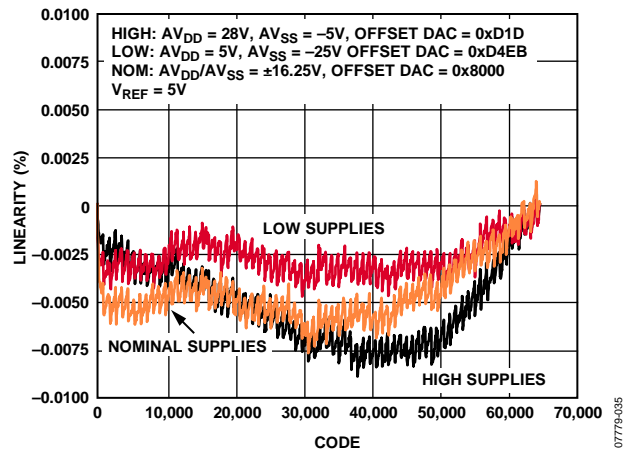
Figure 11. Measure Current Linearity vs. Code (MEASOUT Gain = 1, MI Gain = 20), T_j = 25^\circ C
