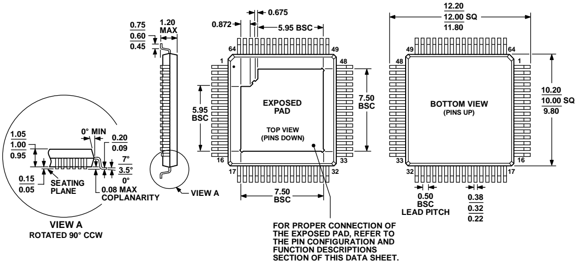
COMPLIANT TO JEDEC STANDARDS MS-026-ACD-HU Figure 59. 64-Lead Thin Quad Flat Package, Exposed Pad [TQFP_EP] (SV-64-3) Dimensions shown in millimeters
