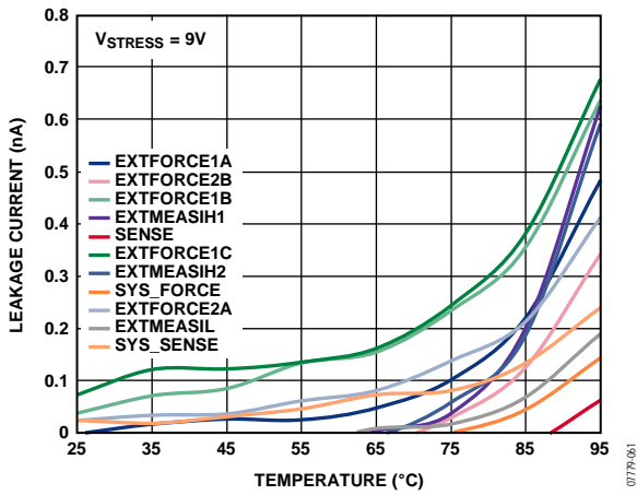
Figure 20. Leakage Current vs. Temperature, V_{STRESS} = 9V
