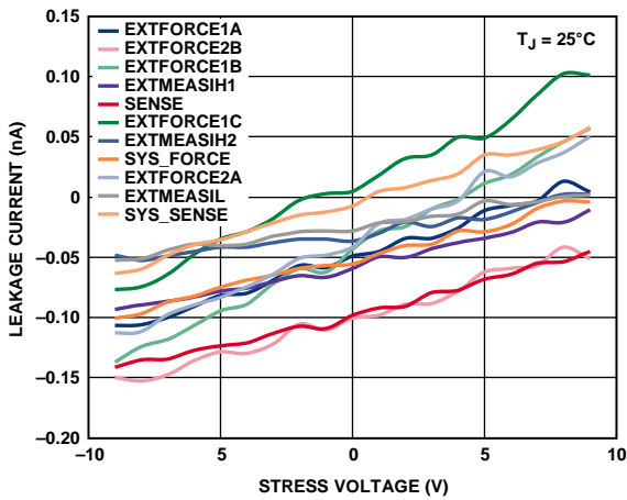
Figure 19. Leakage Current vs. Stress Voltage
