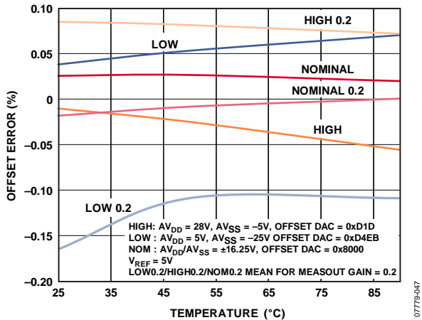
Figure 21. MI Offset Error vs. Temperature, MI Gain = 20, MEASOUT Gain = 1 and 0.2
