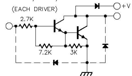
SG2803/2813/2823
