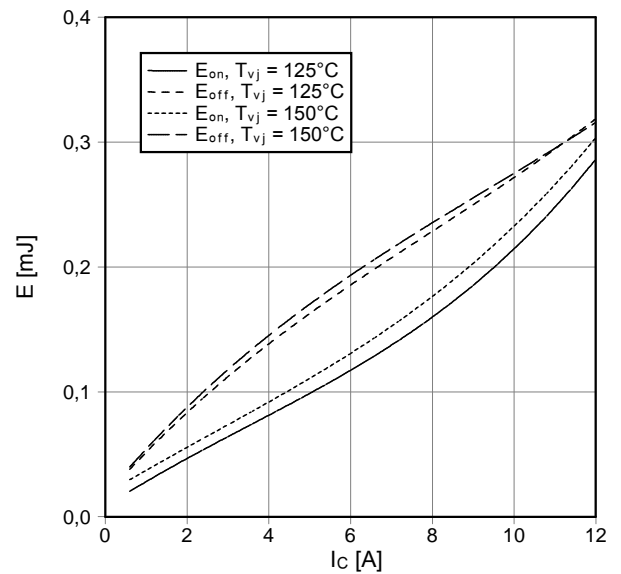
Schaltverluste IGBT-Wechselr. (typisch) switching losses IGBT-inverter (typical) E_{on} = f(I_c), E_{off} = f(I_c) V_{GE} = \pm 15\text{ V}, R_{Gon} = 47\ \Omega, R_{Goff} = 47\ \Omega, V_{CE} = 300\text{ V}
