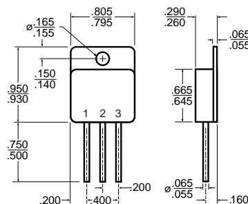
TO-267
