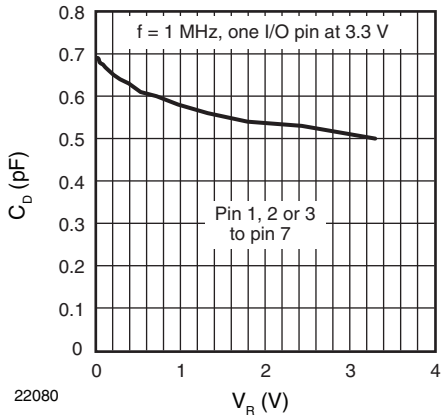
Figure 4. Typical Capacitance C_D vs. Reverse Voltage V_R
