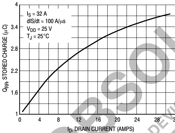
Figure 10. Stored Charge
