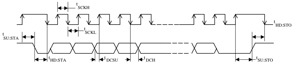
Data interface timing (I 2 C)
