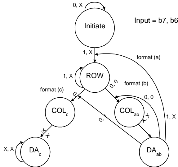
FIGURE 3. Transmission State Diagram
