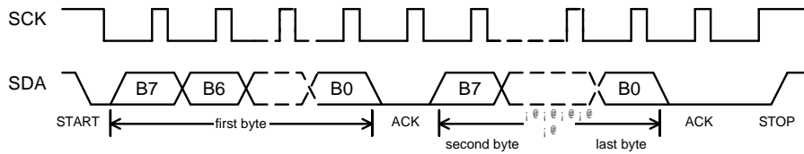
FIGURE 2. Data Transmission Protocol (I 2 C)
