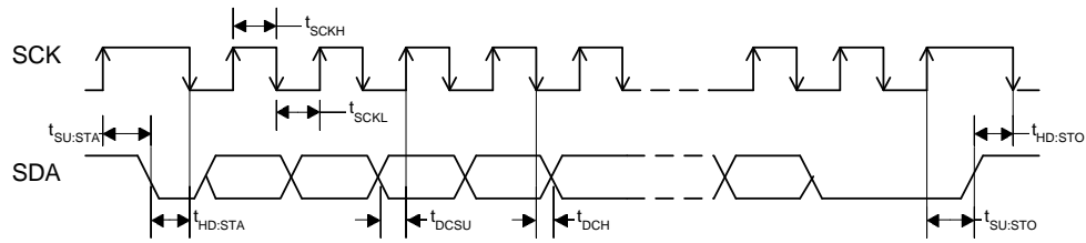
FIGURE 9. Data interface timing(I 2 C)
