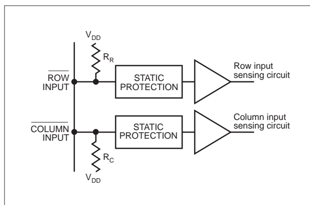
Figure 6: Row and Column inputs
