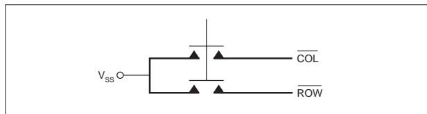
Figure 4: 2 of 8 DTMF keyboard
