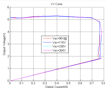
I-V Curve
