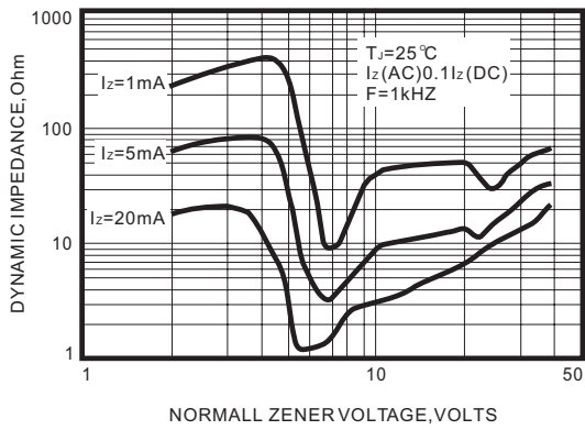
Fig.3 EFFECT OF ZENER VOLTAGE ON ZENER IMPEDANCE
