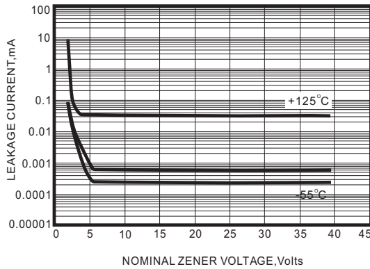
Fig.5 TYPICAL LEAKAGE CURRENT
