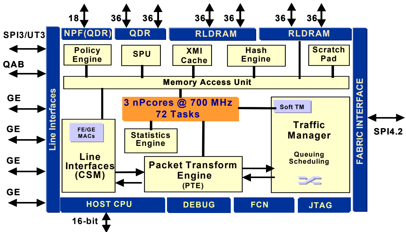
nP3710 Block Diagram
