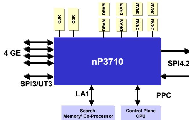
nP3710 Interface Diagram
