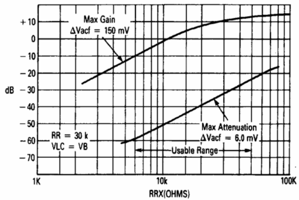
FIGURE 3 — RECEIVE ATTENUATOR versus RRX
