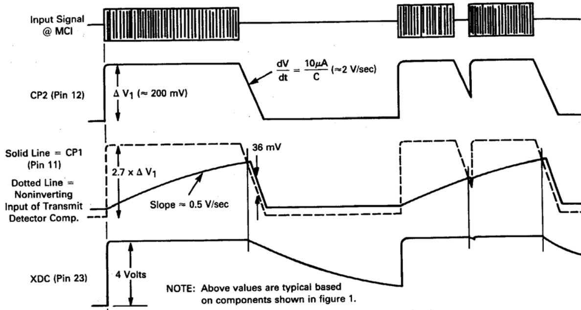
FIGURE 11 — TRANSMIT DETECTOR OPERATION
