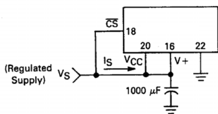
FIGURE 14 — ALTERNATE POWER SUPPLY CONFIGURATION
