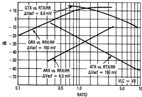
FIGURE 4 — GAIN AND ATTENUATION versus RESISTOR RATIOS
