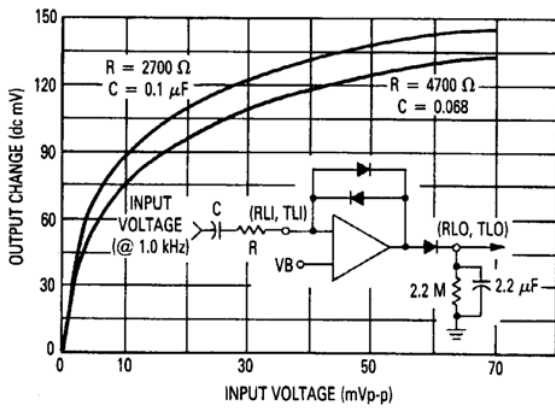
FIGURE 8 — LOG AMP TRANSFER CHARACTERISTICS
