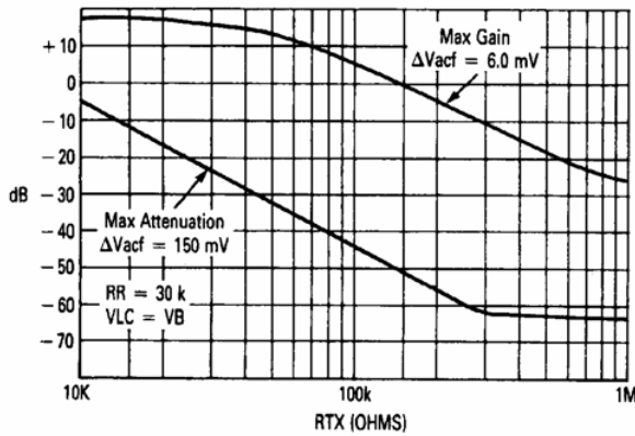
FIGURE 4 — GAIN AND ATTENUATION versus RESISTOR RATIOS
