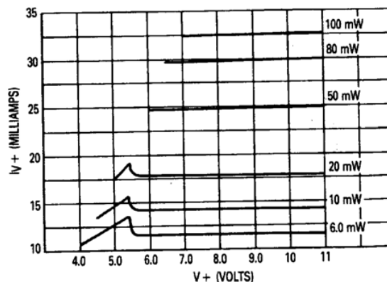
FIGURE 15 — SUPPLY CURRENT versus SUPPLY VOLTAGE (SEE FIGURE 14)
