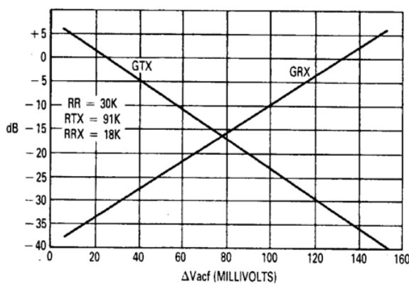
FIGURE 6 — ATTENUATOR GAIN versus \Delta V_{acf}
