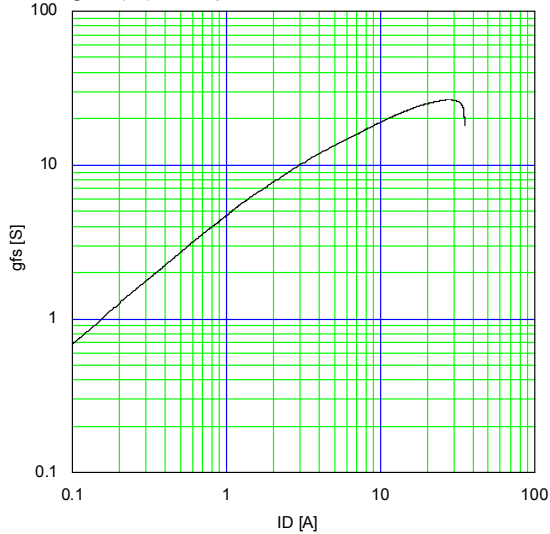
Typical Transconductance g_{fs}=f(I_D):80\ \mu\text{s}\ \text{pulse test},V_{DS}=25\text{V},T_{ch}=25^\circ\text{C}
