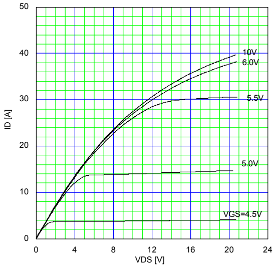
Typical Output Characteristics I_D=f(V_{DS}):80\ \mu\text{s}\ \text{pulse test},T_{ch}=25^\circ\text{C}
