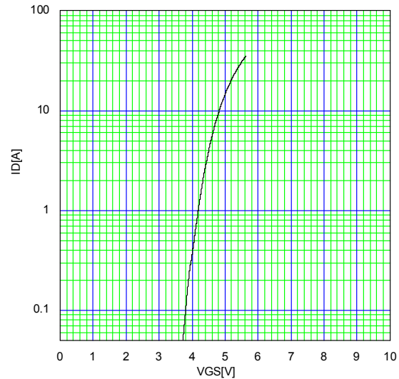
Typical Transfer Characteristic I_D=f(V_{GS}):80\ \mu\text{s}\ \text{pulse test},V_{DS}=25\text{V},T_{ch}=25^\circ\text{C}
