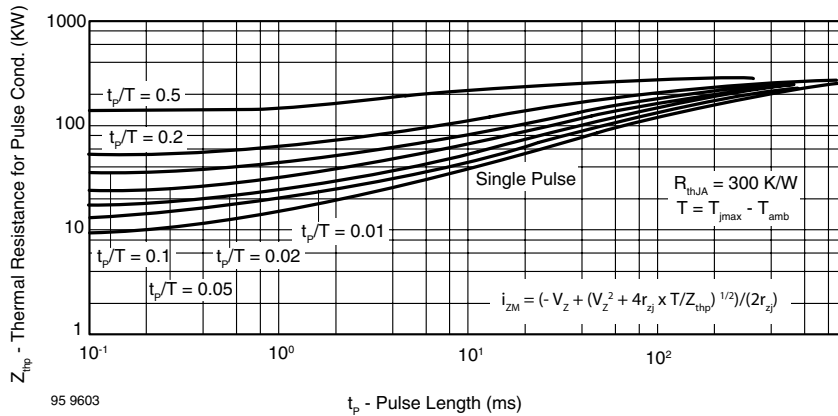
Figure 10. Thermal Response
