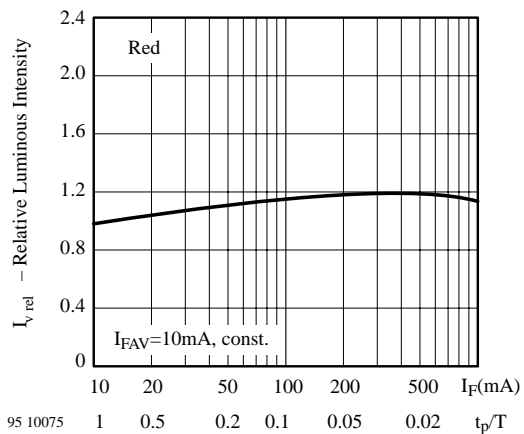
95 10075 I_{F(AV)}=10\text{mA, const.} Figure 6. Rel. Lumin. Intensity vs. Forw. Current/Duty Cycle
