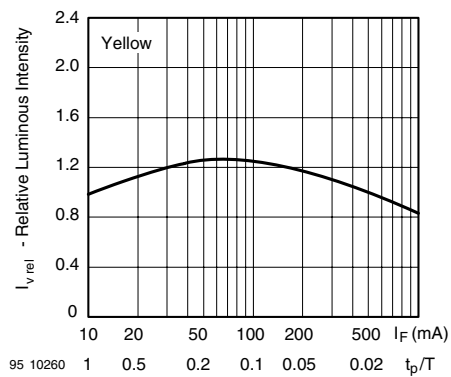
Figure 11. Rel. Lumin. Intensity vs. Forw. Current/Duty Cycle
