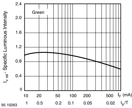
Figure 16. Specific Luminous Intensity vs. Forward Current
