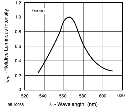
Figure 18. Relative Intensity vs. Wavelength
