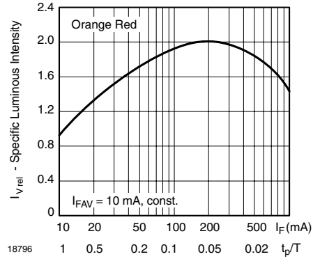
Figure 6. Rel. Lumin. Intensity vs. Forw. Current/Duty Cycle
