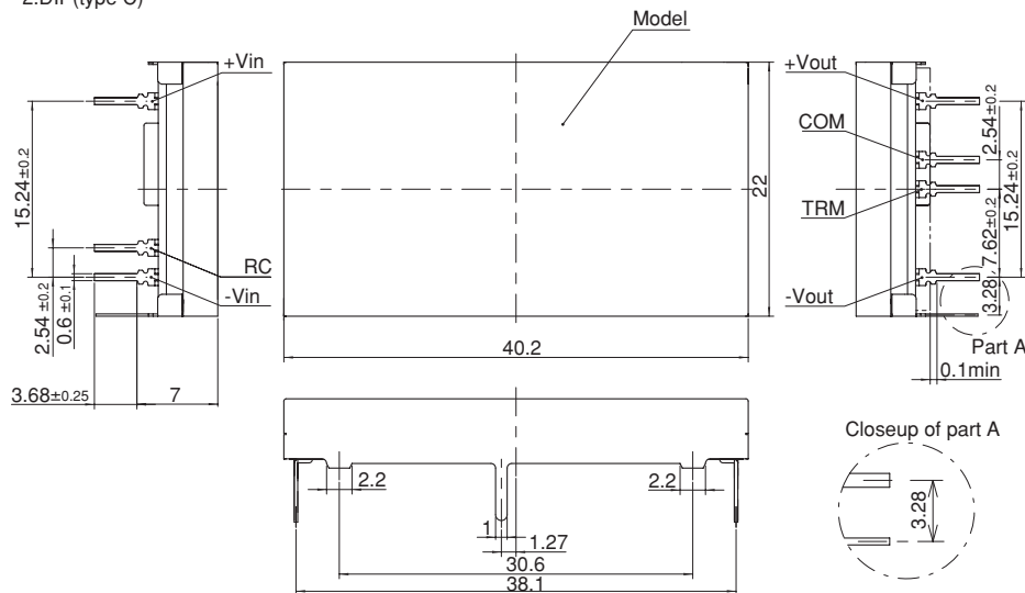
2.DIP(type C)
