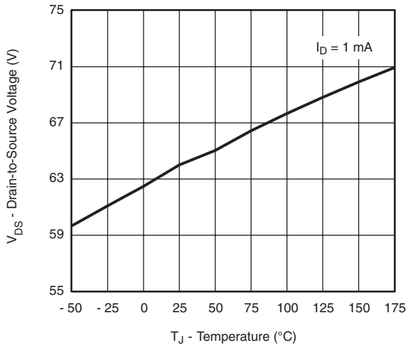
Drain-Source Brakdown vs. Junction Temperature
