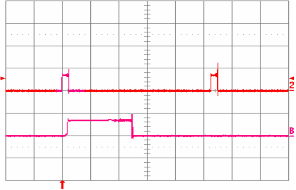
Fig. 6.0V.18: Load current (top trace, 20 A/div., 20 ms/div.) into a 10 mΩ short circuit during restart, at Vin = 24V. Bottom trace (20 A/div., 2 ns/div.) is an expansion of the on-time portion of the top trace.
