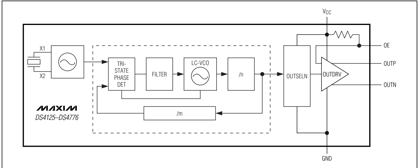
Figure 1. Functional Diagram
