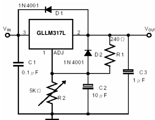
Fig 2. Voltage Regulator with Protection Diodes
