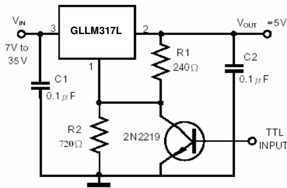
Fig 4. 5V Electronic Shut-Down Regulator
