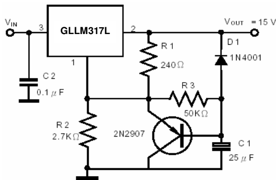
Fig 3. Slow Turn-On 15V Regulator
