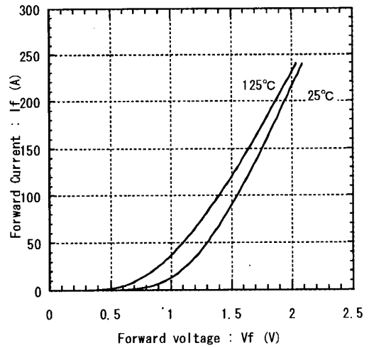
Forward current vs. Forward voltage (Terminal)
