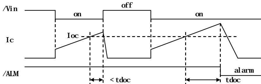
Figure 3. Over-current Protection Timing Diagram
