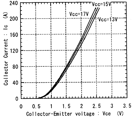
Collector current vs. Collector-Emittter voltage T j =25°C (Terminal)
