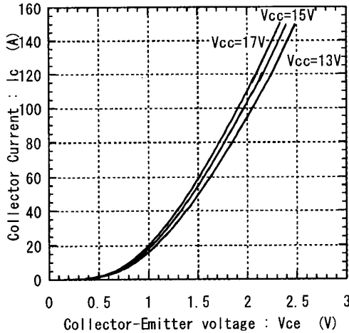
Collector current vs. Collector-Emmitter voltage T j =125°C (Chip)
