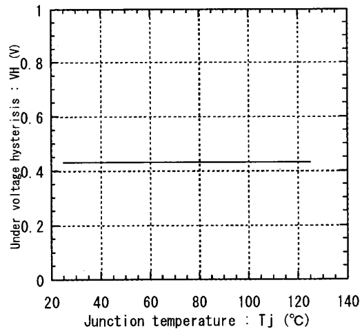
Under voltage hysteresis vs. Junction temperature
