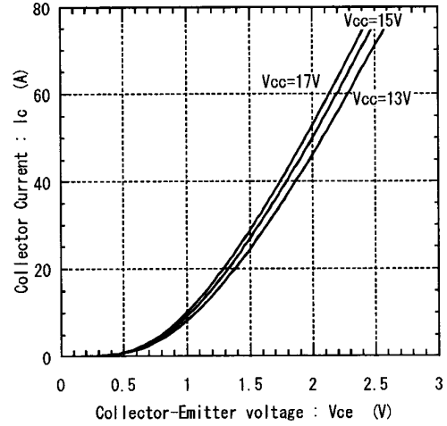
Collector current vs. Collector-Emittor voltage T_j=125^\circ\text{C}
