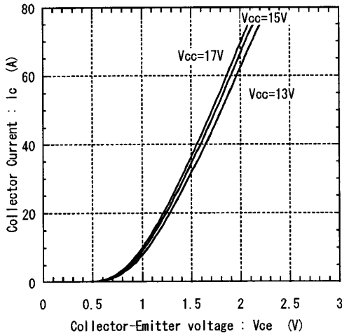
Collector current vs. Collector-Emittor voltage T_j=25^\circ\text{C}
