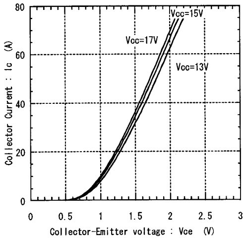
Collector current vs. Collector-Emittor voltage T_j=25^\circ\text{C}
