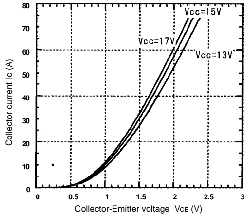
Collector current vs. Collector-Emittter voltage T j =125°C(Chip)
