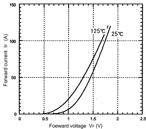
Forward current vs. Forward voltage (Chip)
