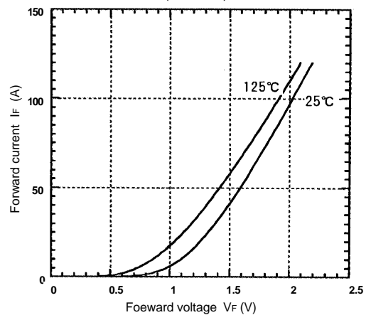
Forward current vs. Forward voltage (Terminal)
