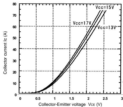
Collector current vs. Collector-Emittter voltage T j =125°C(Terminal)
