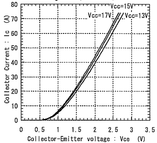
Collector current vs. Collector-Emittor voltage T j =25°C (Terminal)
