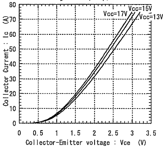
Collector current vs. Collector-Emittor voltage T j =125°C (Chip)
