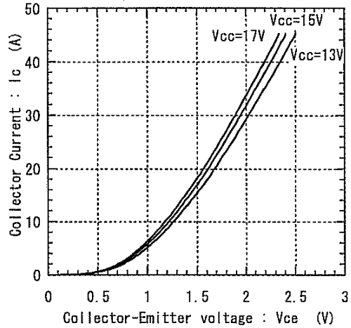
Collector current vs. Collector-Emittter voltage T_j=125^{\circ}\text{C} (Terminal)
