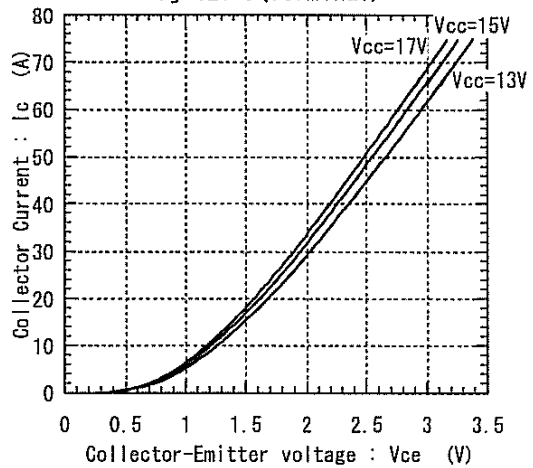
Collector current vs. Collector-Emittor voltage T j =125°C (Terminal)
