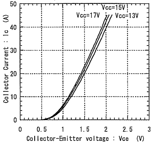
Collector current vs. Collector-Emittter voltage T_j=25^{\circ}\text{C} (Terminal)
