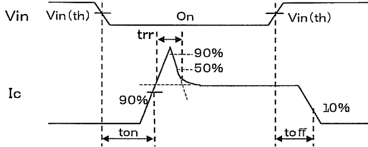
Figure 1. Switching Time Waveform Definitions
