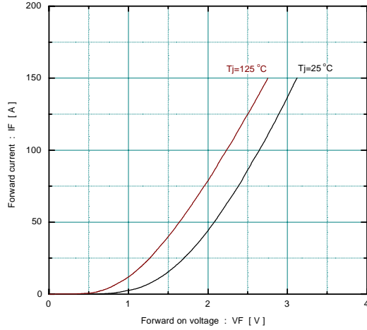
Forward current vs. Forward on voltage (typ.)
