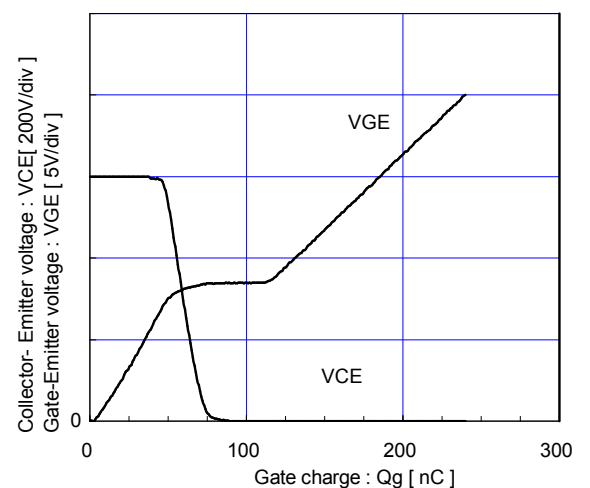
Dynamic Gate charge (typ.) Vcc=600V, Ic=50A, Tj=25°C
