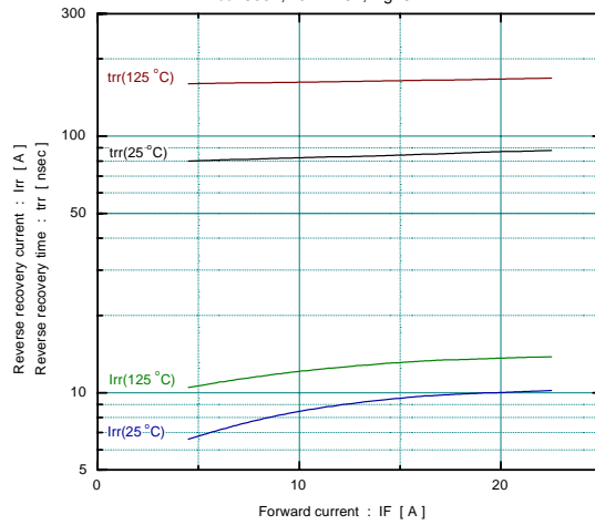
Reverse recovery characteristics (typ.) V CC =600V, V GE ±15V, R G =82Ω
