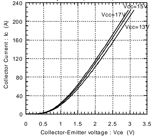
Collector current vs. Collector-Emittter voltage Tj=125°C(Terminal)
