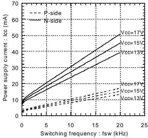
Power supply current vs. Switching frequency Tc=125°C
