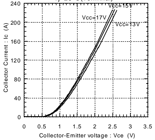
Collector current vs. Collector-Emittter voltage Tj=25°C(Terminal)
