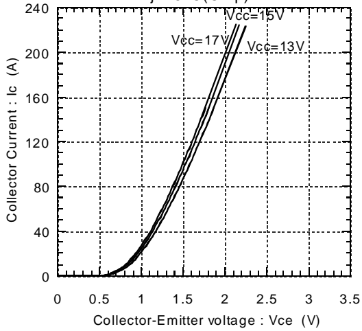
Collector current vs. Collector-Emittter voltage Tj=25°C(Chip)
