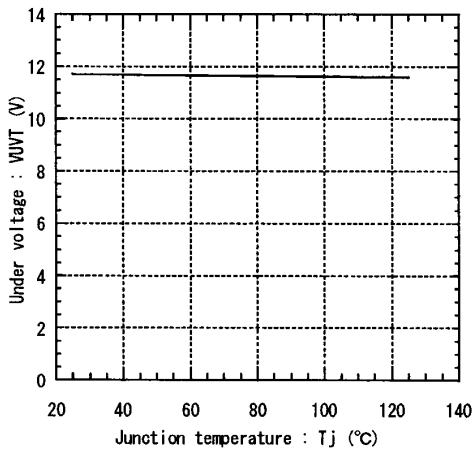
Under voltage vs. Junction temperature
