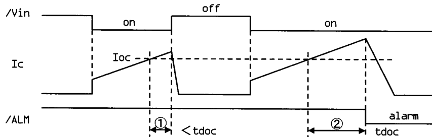
Figure 3. Over-current Protection Timing Diagram
