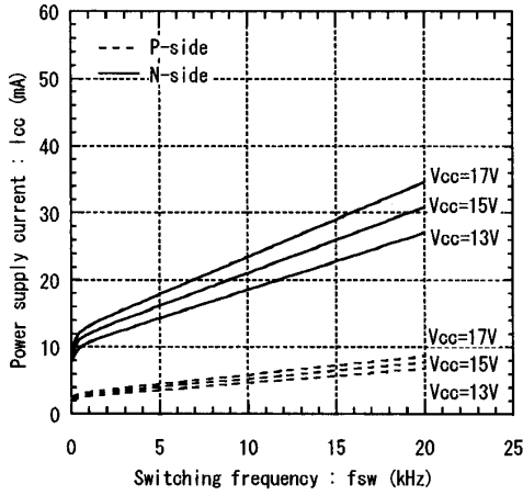
Power supply current vs. Switching frequency Tc=125°C
