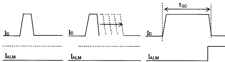
Figure.4 Definition of tsc
