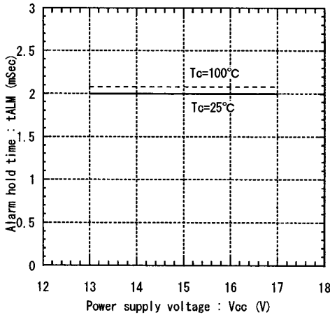
Alarm hold time vs. Power supply voltage
