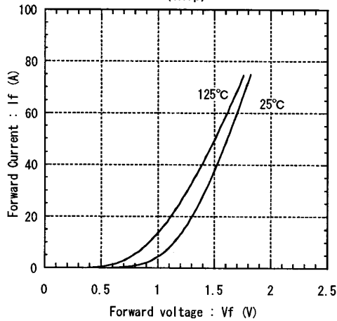
Forward current vs. Forward voltage (Chip)
