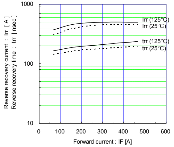
Reverse recovery characteristics (typ.) Vcc=900V, VGE=±15V, Rg=1.5Ω
