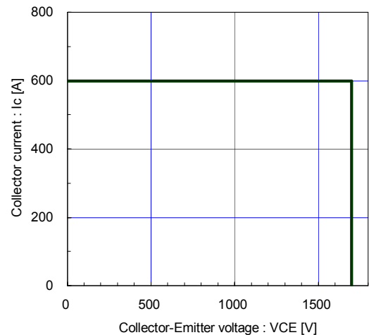
Reverse bias safe operating area (max.) +V_{GE}=15V, -V_{GE} \le 15V, R_g \ge 1.5\Omega, T_j \le 125^\circ C
