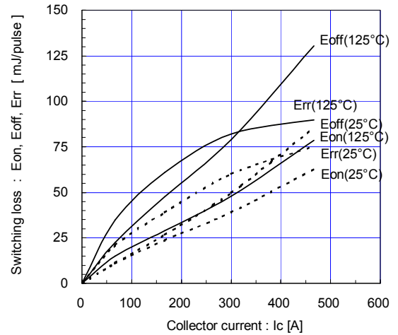
Switching loss vs. Collector current (typ.) V_{cc}=900V, V_{GE}=\pm 15V, R_g=1.5\Omega
