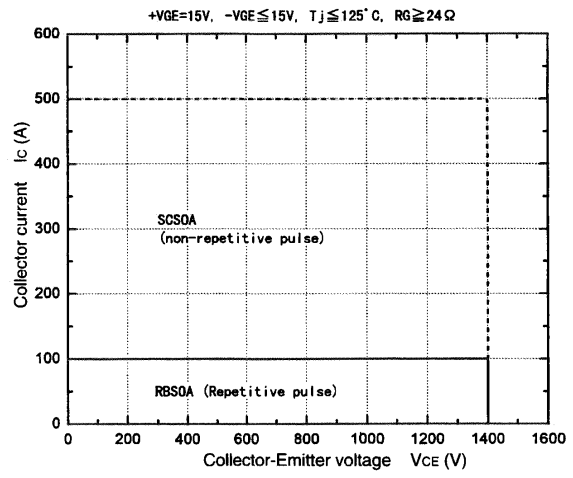
Reverse biased safe operating area
