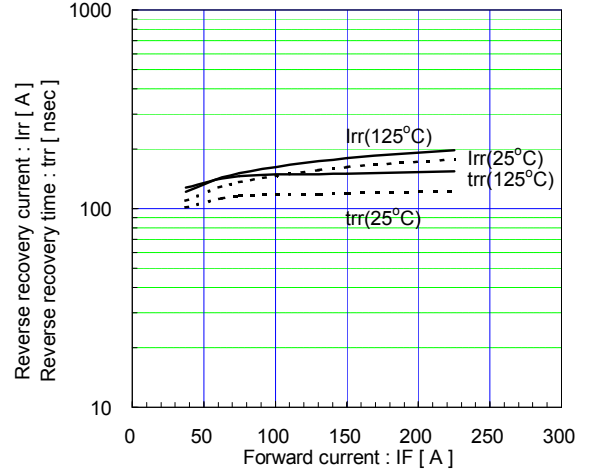
Reverse recovery characteristics (typ.) Vcc=600V, VGE=±15V, RG=4.7Ω
