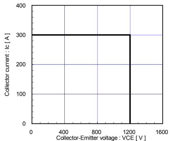
Reverse bias safe operating area (max.) +V_{GE}=15V, -V_{GE} \le 15V, R_G \ge 4.7\Omega, T_J \le 125^\circ C
